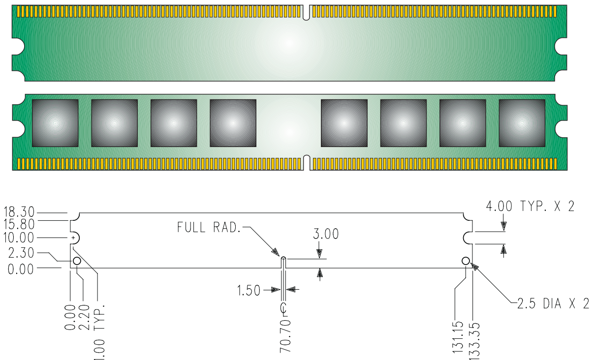
Figure 1: KVR800D2N5/1G 240-Pin DIMM
