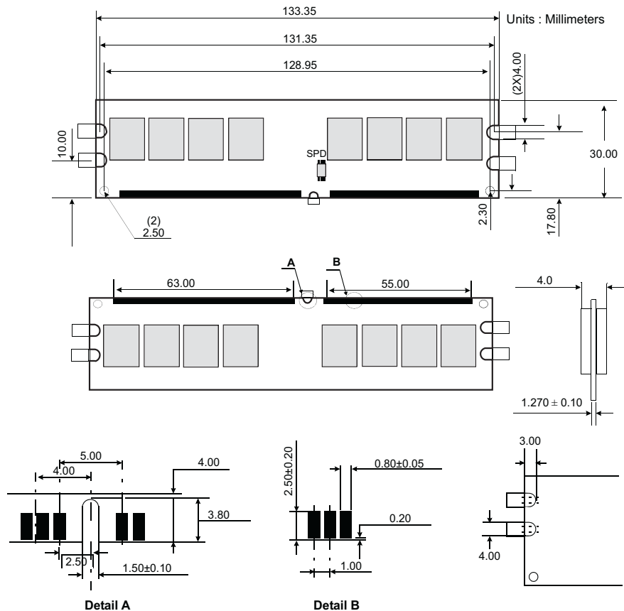
Figure 1: KVR400D2N3/2G 240-Pin DIMM
