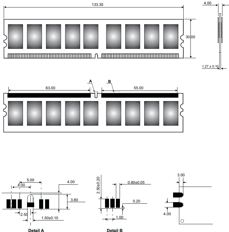
Figure 1: KVR400D2E3/2G 240-Pin DIMM
