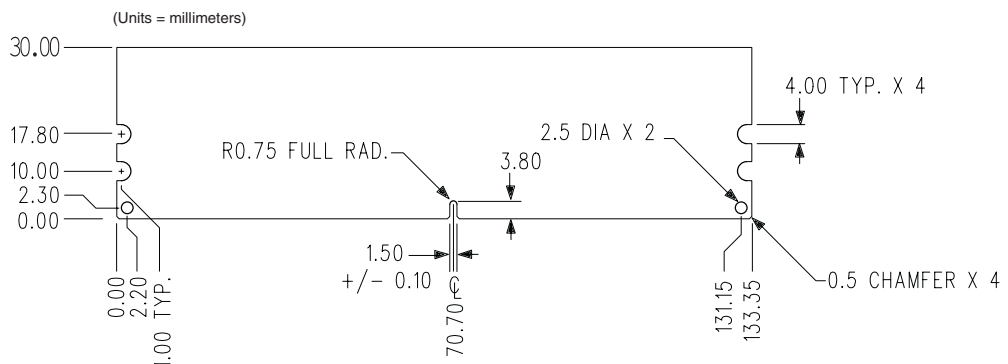
Figure 1: KVR400D2D4R3/4GI 240-Pin DIMM
