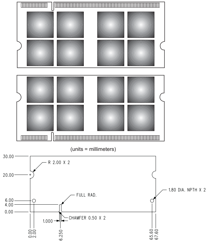
Figure 1: KVR533D2S4/1G 200-Pin SODIMM
