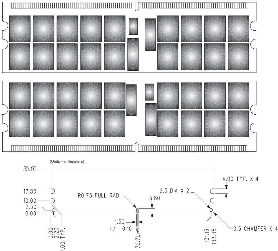
Figure 1: KVR533D2Q8R4/4G 240-Pin DIMM
