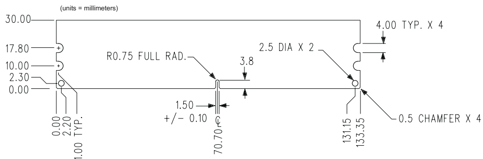
Figure 1: KVR667D2S4P5/2G 240-Pin DIMM
