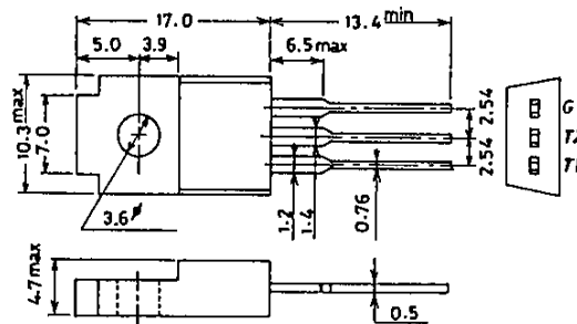
Package Dimensions 1144 (unit: mm)
