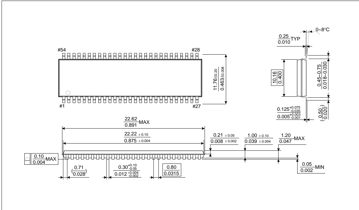
54Pin TSOP Package Dimension
