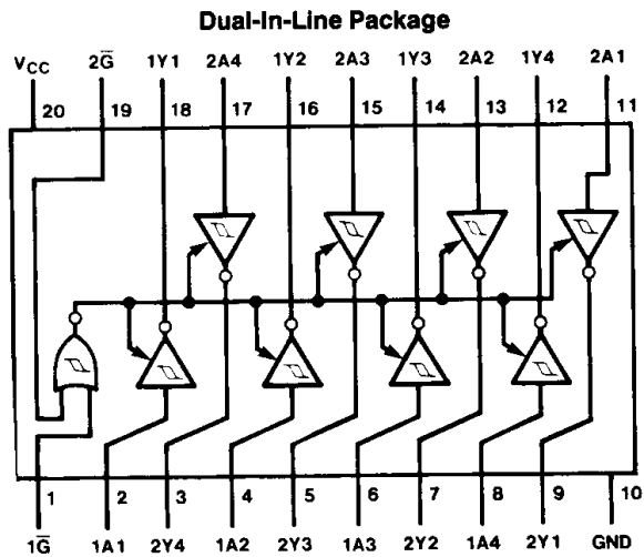
Order Number DM54S940J or 74S940N See NS Package Number J20A or N20A
