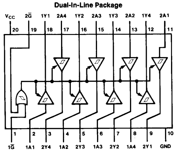
Order Number DM54S941J or 74S941N See NS Package Number J20A or N20A
