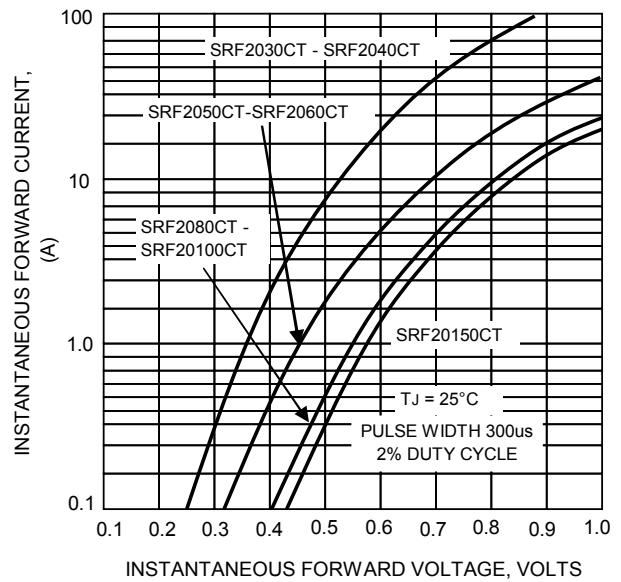
FIG.4-TYPICAL FORWARD CHARACTERISTICS
