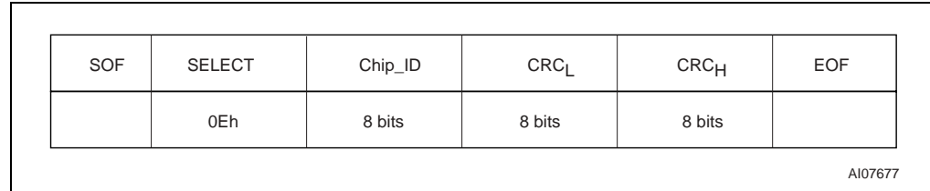
Figure 30. SELECT request format
