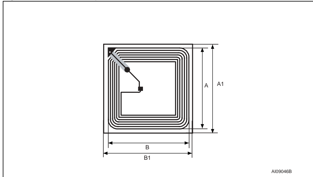
Figure 50. A3 antenna specification
