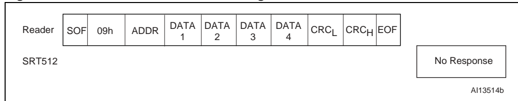
Figure 44. WRITE_BLOCK frame exchange between Reader and SRT512
