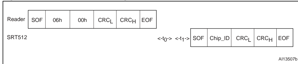
Figure 53. INITIATE frame exchange between Reader and SRT512
