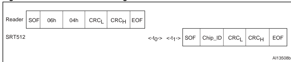
Figure 55. SLOT_MARKER frame exchange between Reader and SRT512
