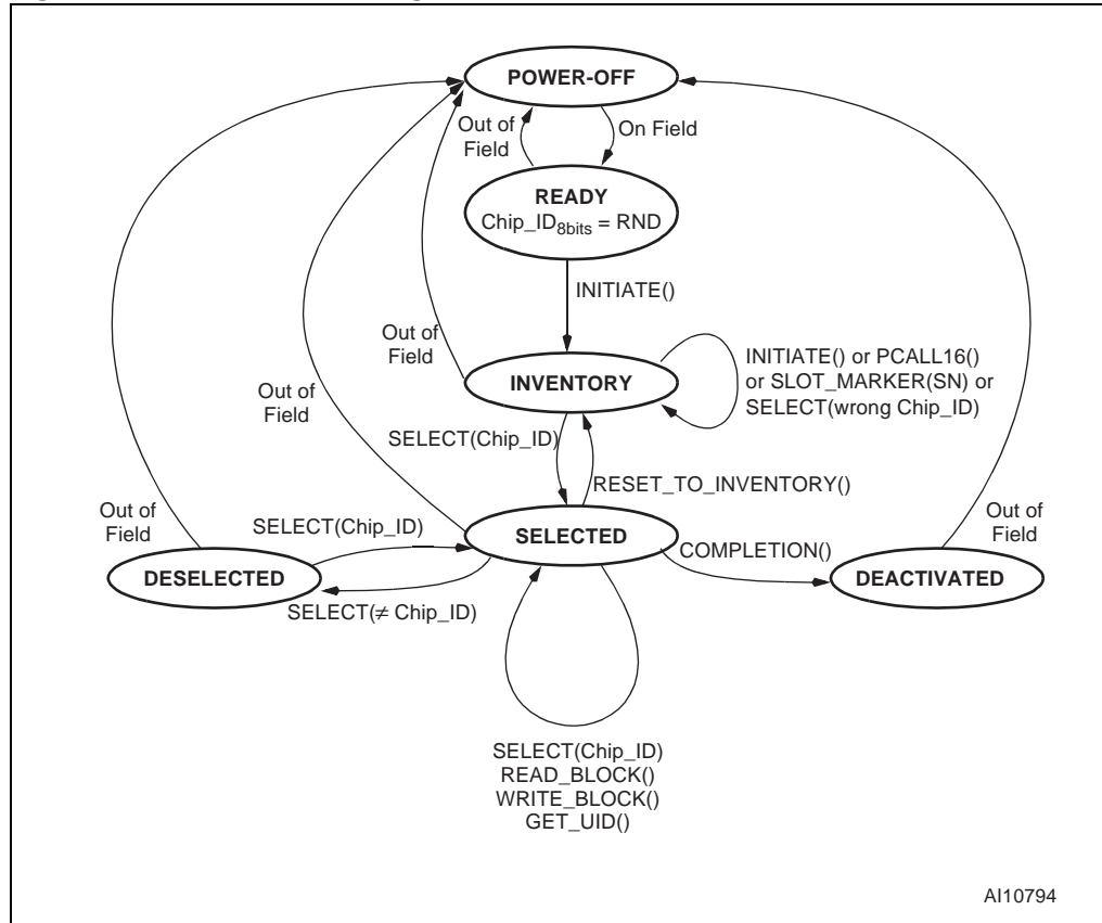
Figure 17. State transition diagram
