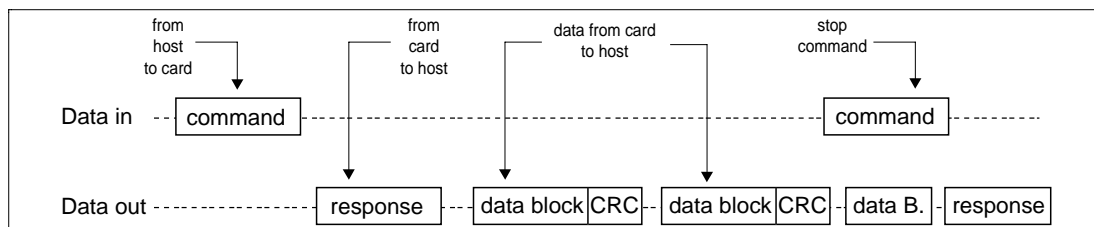
Multiple Block Read Operation
