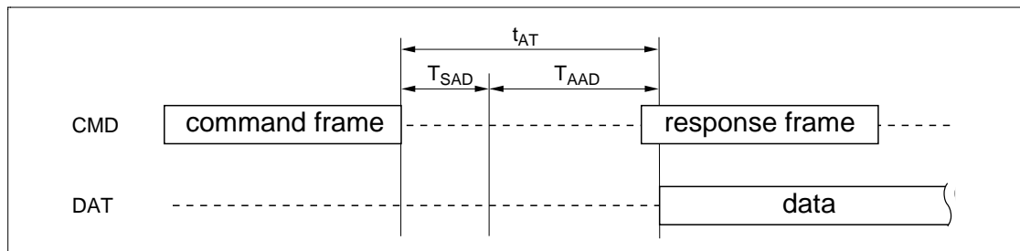
Access Time
