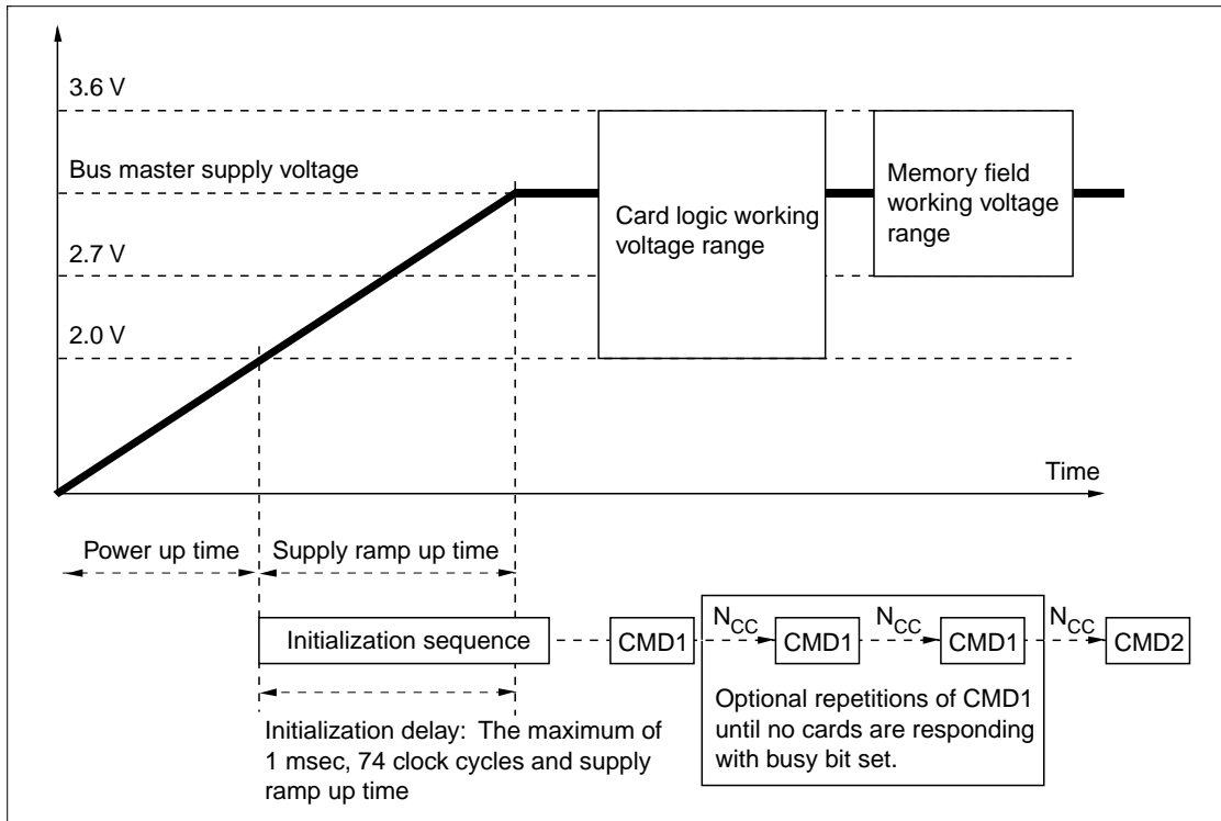
Power-up Diagram
