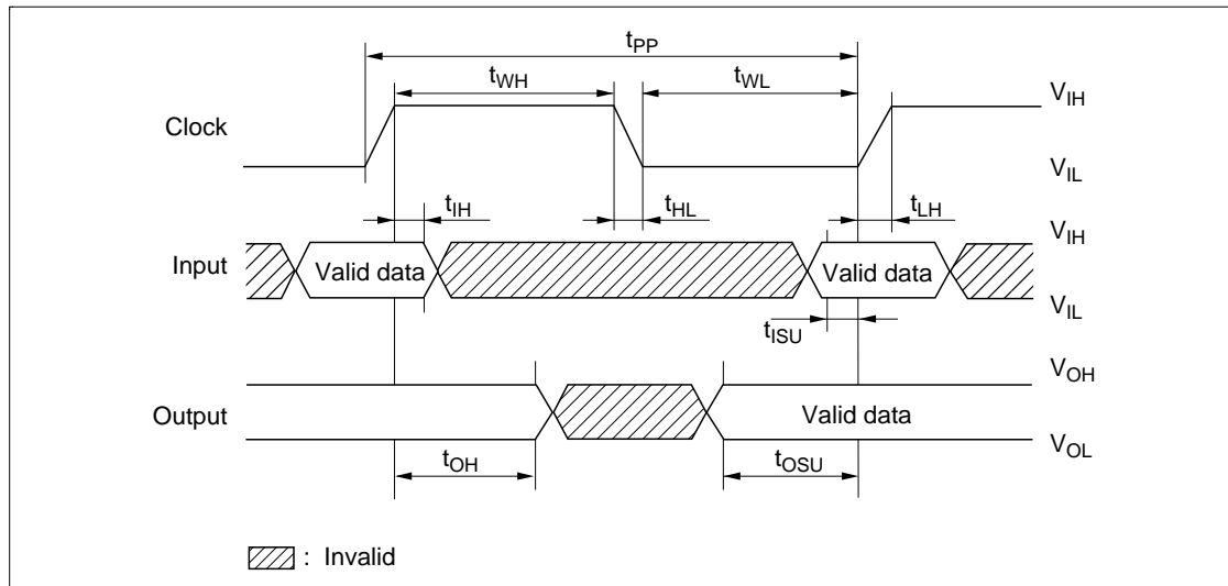
Timing Diagram of Data Input and Output
