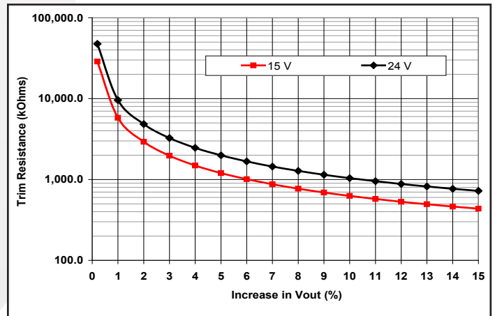
Common Figure 4: Trim graph for trim-up 12 to 24 V outputs.
