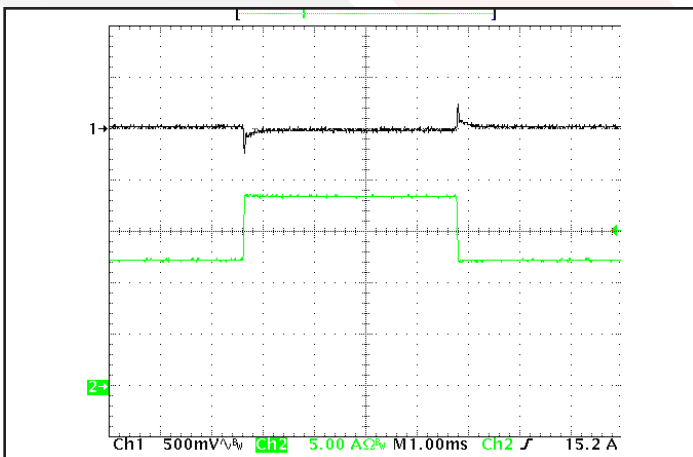
Figure 5: Output voltage response to step-change in load current (50%-75%-50% of I out (max); dl/dt = 0.1A/μs). Load cap: 15μF tantalum cap and 1μF ceramic cap. Ch 1: V out , Ch 2: I out .
