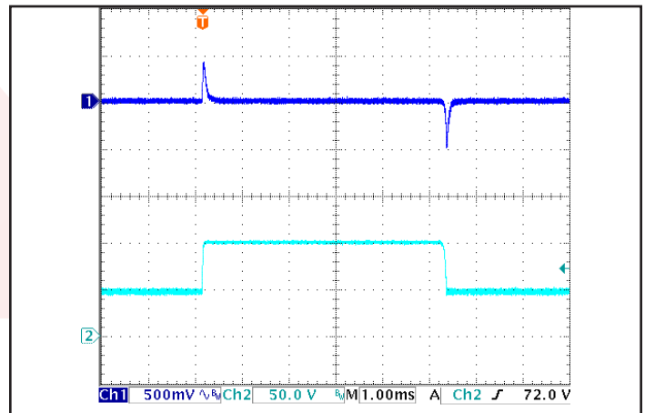
Figure 6: Output voltage response to step-change in input voltage (nominal to maximum input voltage), at full load current. Load cap: uF ceramic cap. Ch 1: V out , Ch 2: V in .
