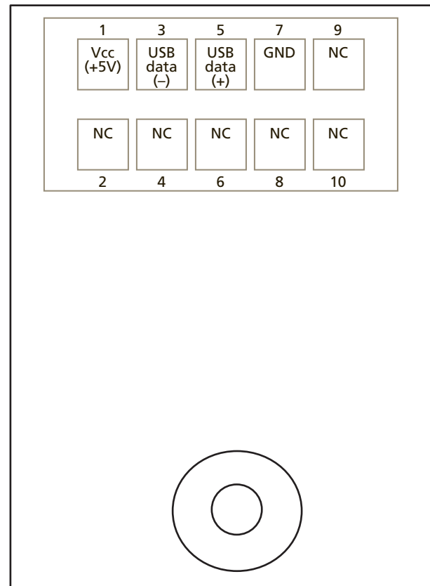
Bottom view
