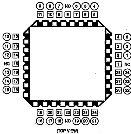
24-Lead Logio Pinout for 28 Terminal Chip Carrier
