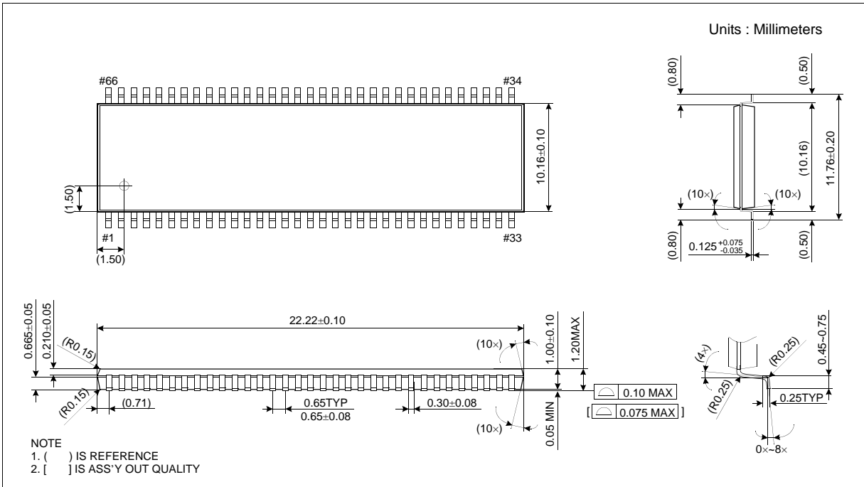
66pin TSOP / Package dimension
