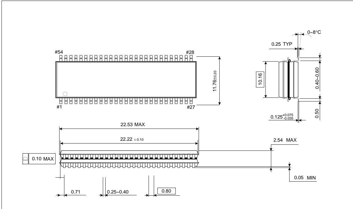
54Pin TSOP2 Stack Package Dimension
