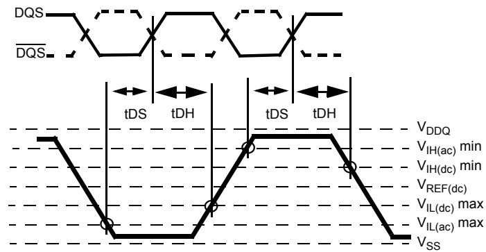
Figure 18 - Differential input waveform timing - t_{DS} and t_{DH}
