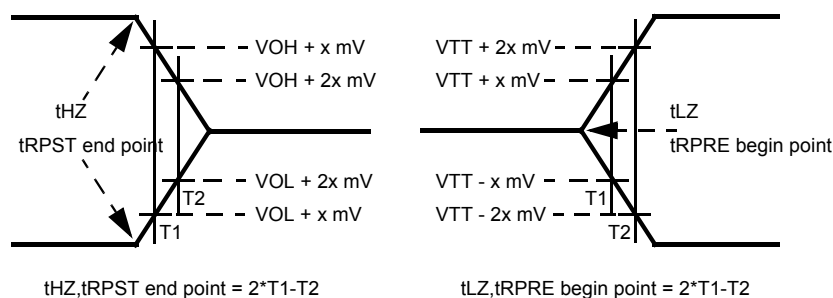
Figure 17 - Method for calculating transitions and endpoints
