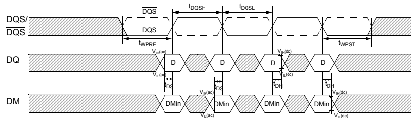
Figure 3 - Data Input (Write) Timing
