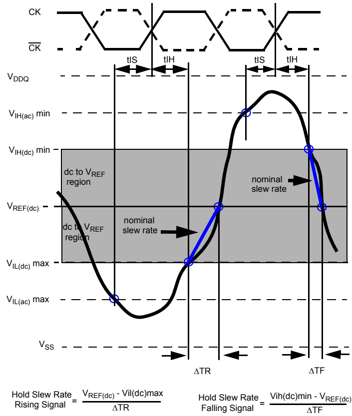
Figure 15 - Illustration of nominal slew rate for tIH
