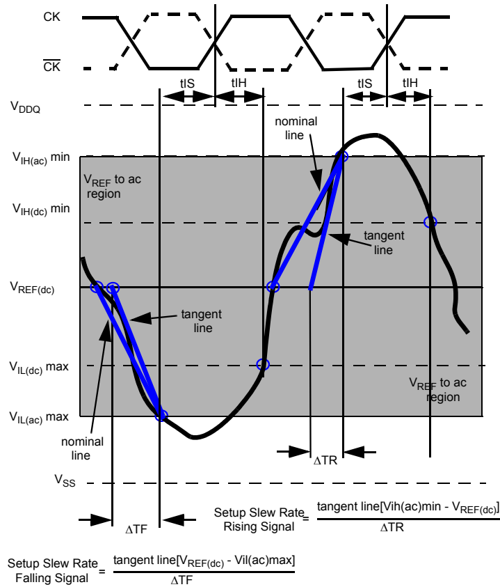
Figure 14 - Illustration of tangent line for tIS
