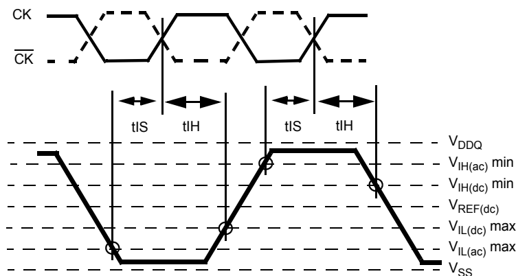
Figure 19 - Differential input waveform timing - t_{IS} and t_{IH}
