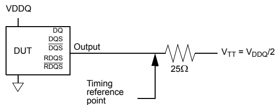
Figure 1 - AC Timing Reference Load
