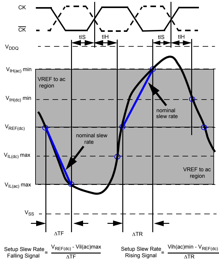
Figure 13 - Illustration of nominal slew rate for tIS
