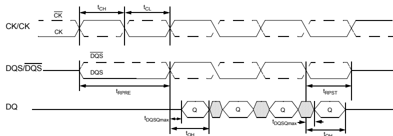
Figure 4 - Data Output (Read) Timing
