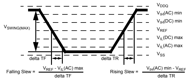
< AC Input Test Signal Waveform >
