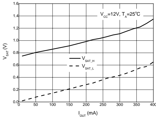
Figure 6. Saturation Voltage vs. Output Current
