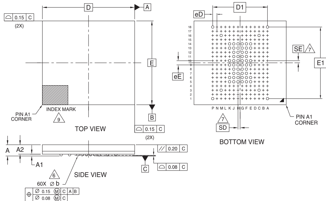
Figure 4.5 NLA060—60-ball VFBGA
