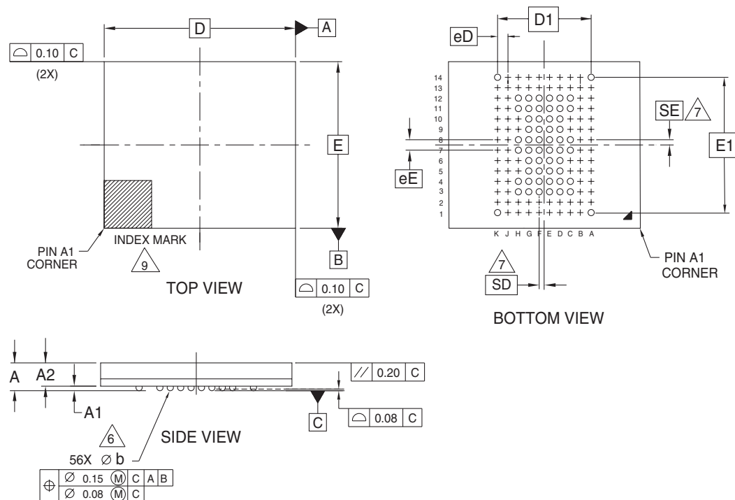
Figure 4.4 NLB056—56-ball VFBGA
