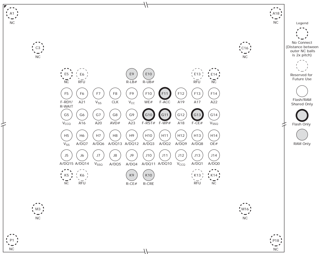
Figure 4.2 pSRAM Based Pinout, 60-Ball, VFBGA
