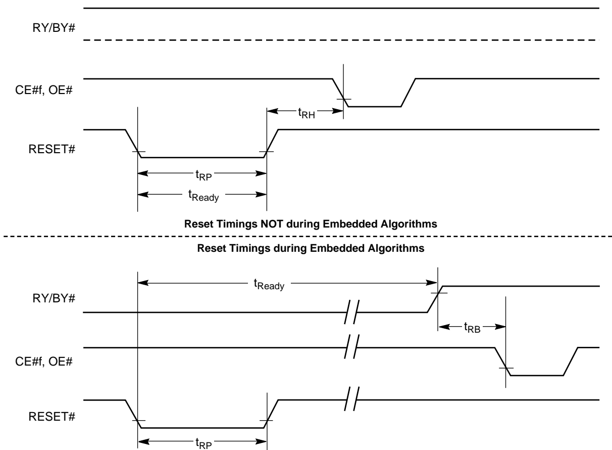
Figure 15. Reset Timings
