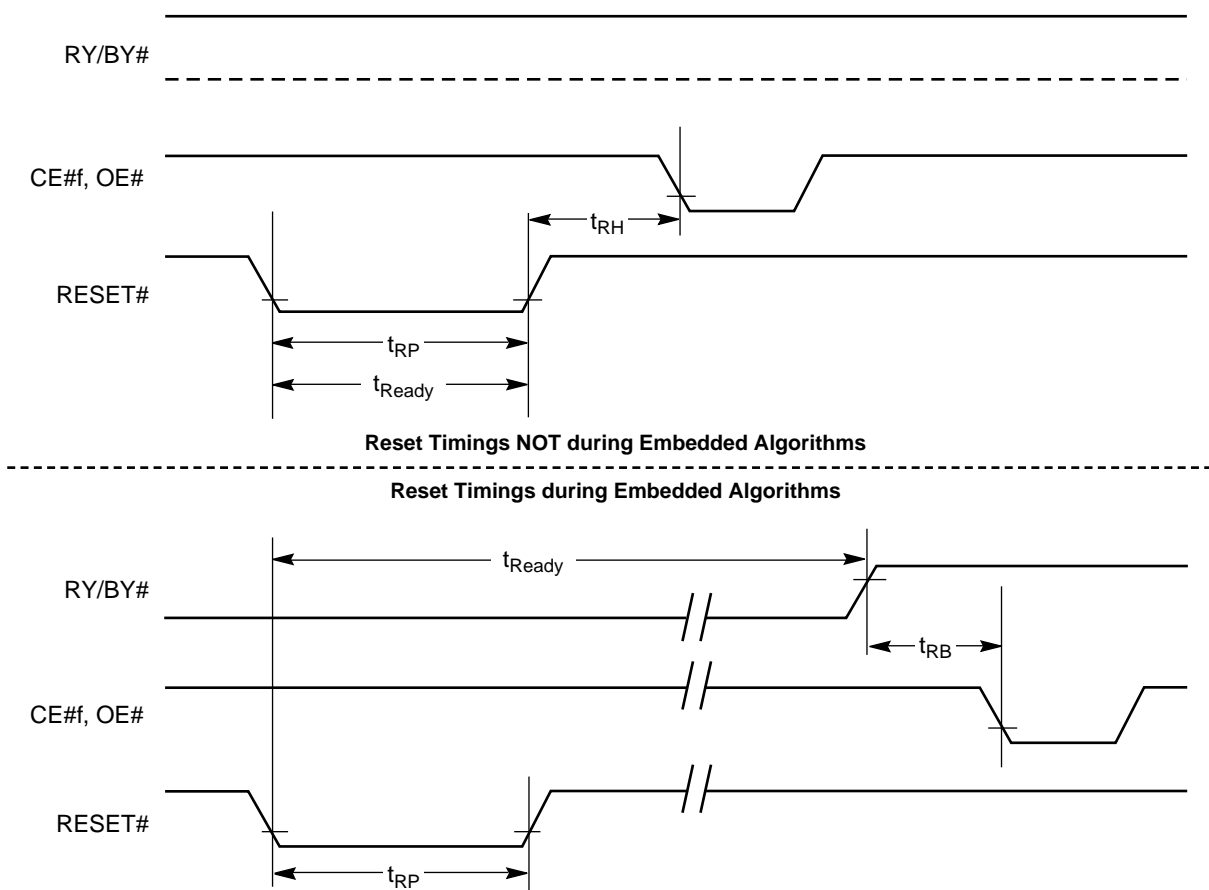
Figure 15. Reset Timings
