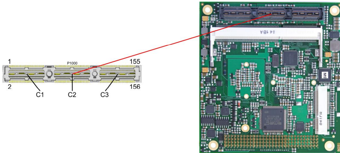
Pinout PCI104-Express connector (type 2):
