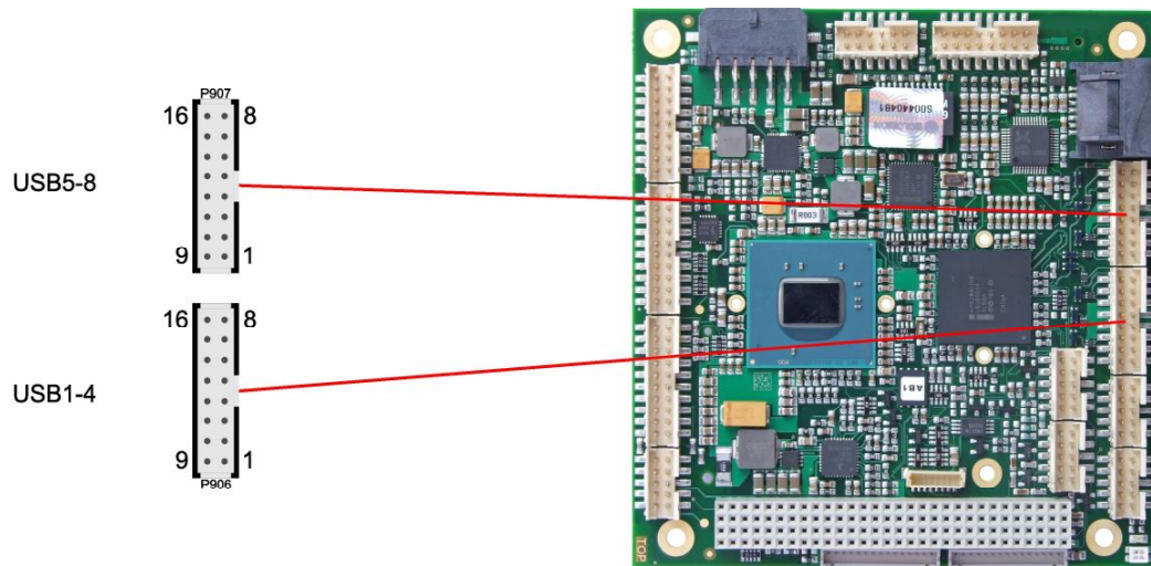
Pinout USB 1-4:
