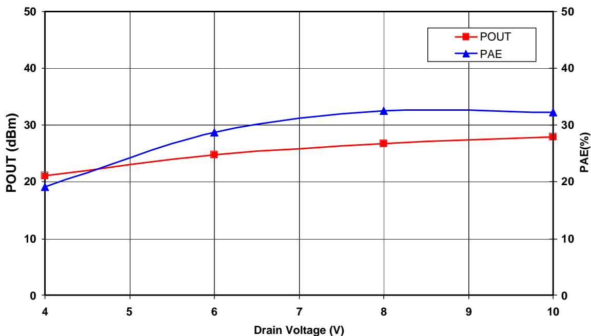
Figure 2. Saturated Output Power and Power Added Efficiency vs. Drain Voltage at f_0 = 10 GHz.
