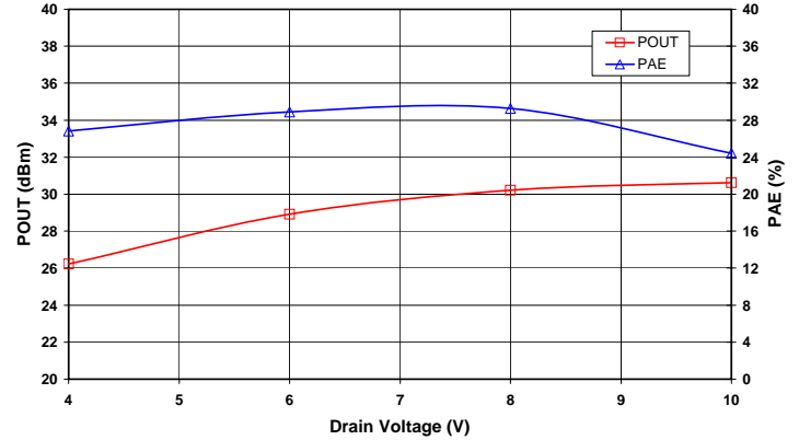
Figure 2. Saturated Output Power and Power Added Efficiency vs. Drain Voltage at f_o = 9.5\text{ GHz} .
