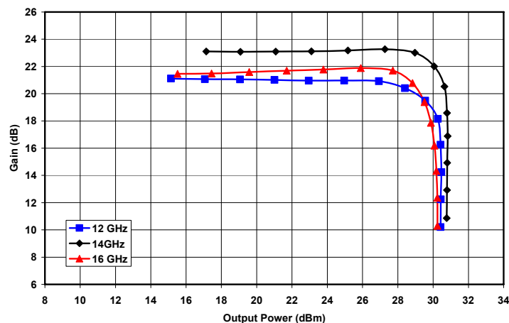
Figure 10. Gain vs. Output Power and Frequency at VD = 8V and IDQ = 470mA
