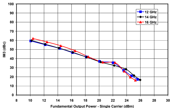
Figure 22. Third Order Intermod vs. Output Power and Frequency at VD = 8V and IDQ = 470mA
