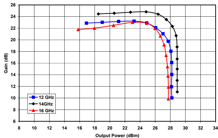
Figure 8. Gain vs. Output Power and Frequency at VD = 6V and IDQ = 470mA
