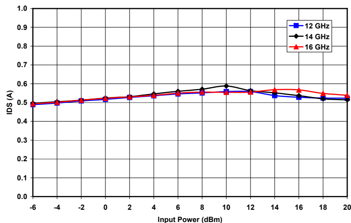
Figure 16. Drain Current vs. Input Power and Frequency at VD = 8V and IDQ = 470mA
