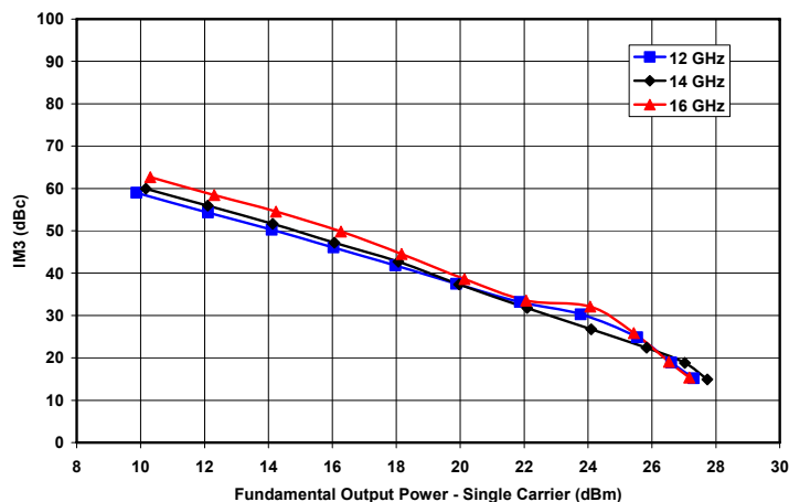
Figure 24. Third Order Intermod vs. Output Power and Frequency at VD = 10V and IDQ = 470mA
