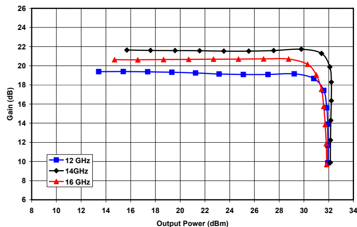
Figure 12. Gain vs. Output Power and Frequency at VD = 10V and IDQ = 470mA
