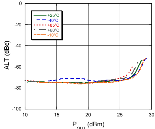
ALT vs. P_{OUT} @ 1905 MHz
