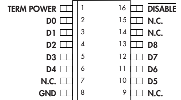
DW PACKAGE (Top View)
