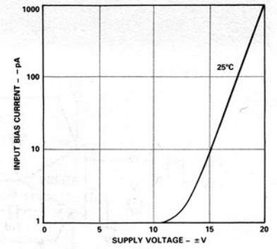
Figure 15. Input Bias Current vs. Supply Voltage
