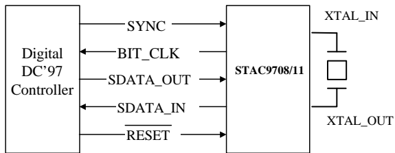
Figure 4. STAC9708/11's AC-Link to its companion controller
