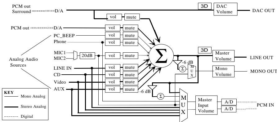
Figure 11. STAC9708/11 Mixer Functional Diagram
