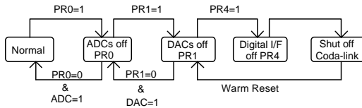
Figure 13. STAC9708/11 Powerdown/Powerup flow with analog still alive
