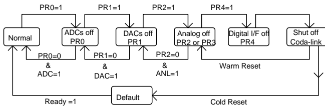
Figure 12. Example of STAC9708/11 Powerdown/Powerup flow
