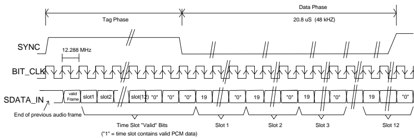
Figure 8. STAC9708/11 Audio Input Frame
