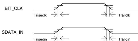
Figure 18. Signal Rise and Fall Times
