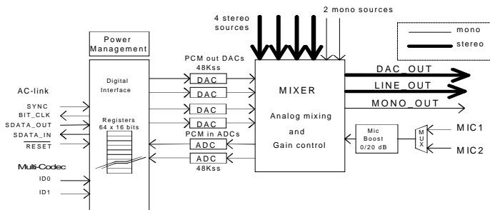
Figure 2. STAC9708 Block Diagram
