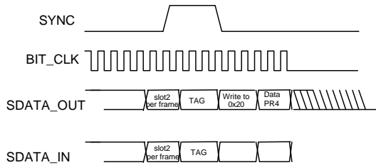
Figure 10. STAC9708/11 Powerdown Timing
