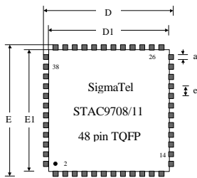
Figure 1. Package Outline
