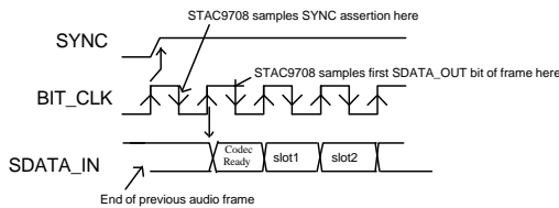
Figure 9. Start of an Audio Input Frame
