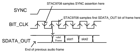
Figure 7. Start of an Audio Output Frame
