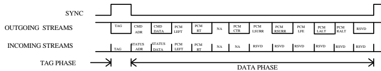
Figure 5. AC'97 Standard Bi-directional Audio Frame
