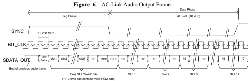
Figure 6. AC-Link Audio Output Frame
