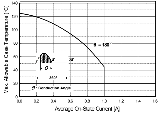
Fig 4. Thermal Response
