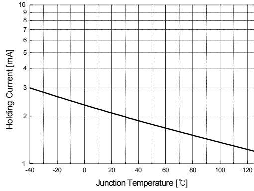
Fig 7. Typical Holding Current
