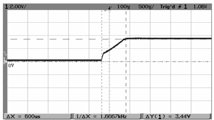
V in = 12V @ FL TURN ON TIME W30-12S3.3
