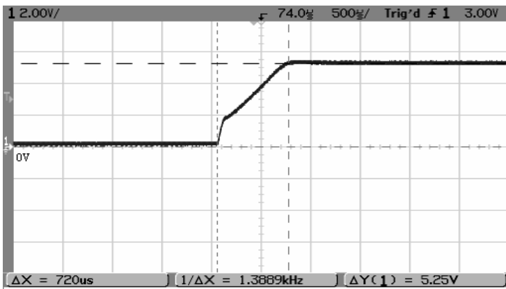
V in = 12V @ FL TURN ON TIME W30-12S5
