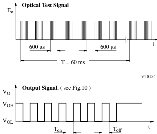
Figure 8. Output Function
