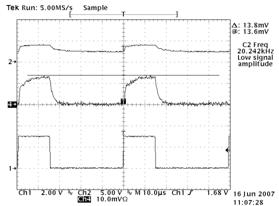
PWM Minimum Duty Cycle 15µs Single LED 20kHz CH1: PWM Signal CH2 Anode of LED CH4: LED current 50mA/div
