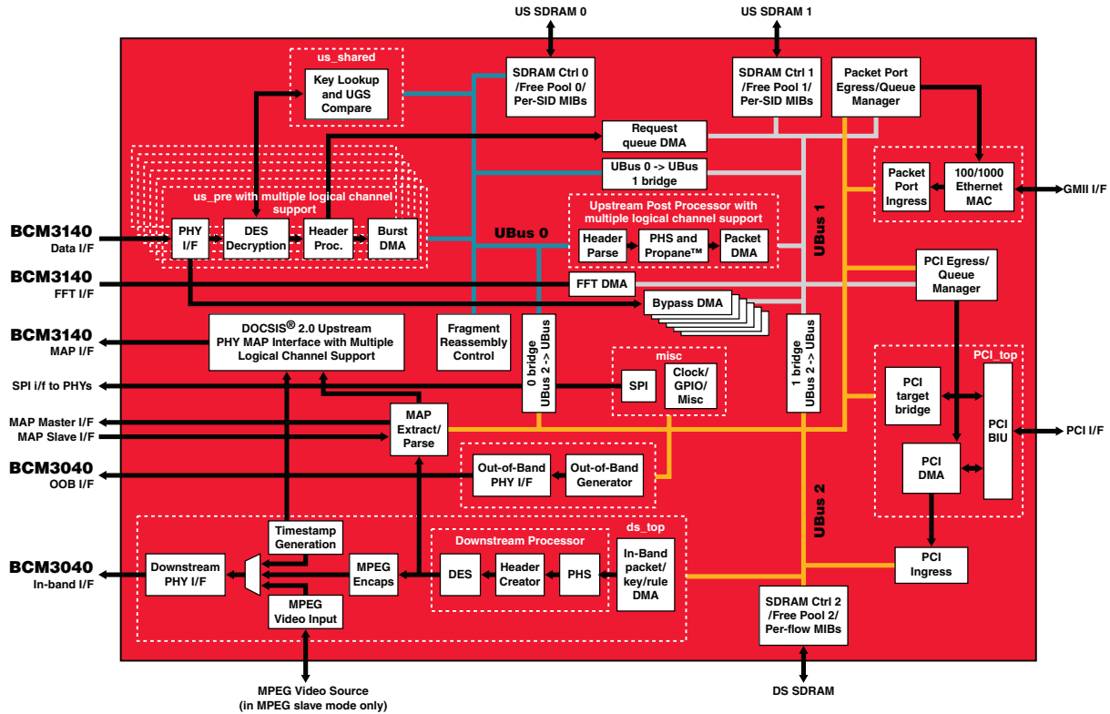
BCM3214 Block Diagram
