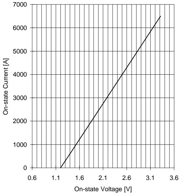
ON-STATE CHARACTERISTIC T j = 125 °C
