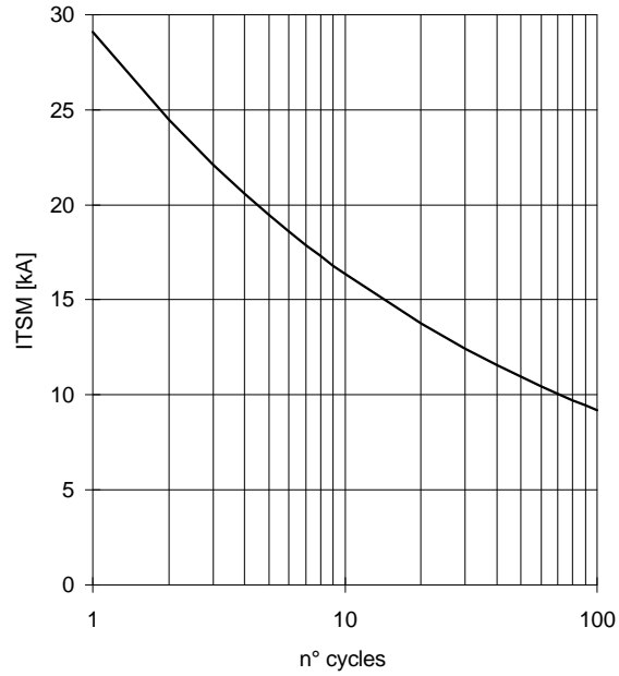
SURGE CHARACTERISTIC T j = 125 °C
