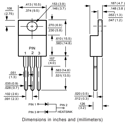
TO-220
