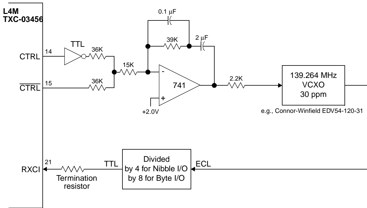
Figure 25. Phase-Locked Loop
