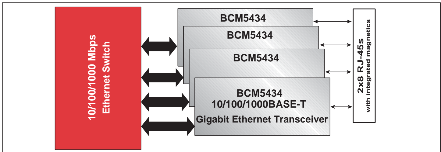
BCM5434 System Diagram
