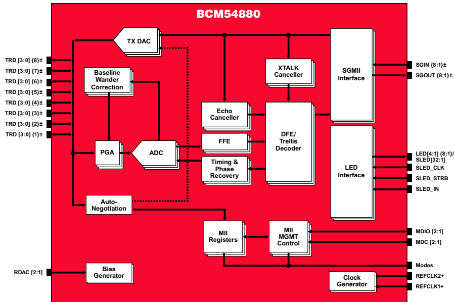
Block Diagram
