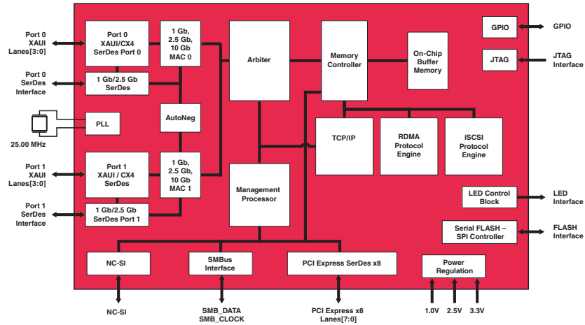
BCM57711 Block Diagram
