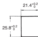
Panel Cutout
