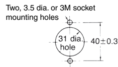
Mounting Holes
