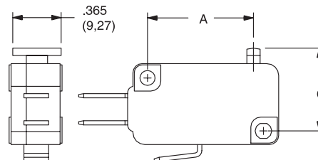
FIG. 5 Wide Pin
