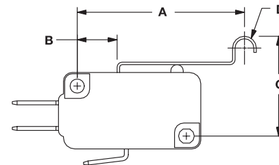
FIG. 4 Simulated Roller
