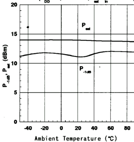
P_{-1dB}, P_{sat} vs. TEMPERATURE ( V_{DD}=3V, f=1.9GHz, P_{sat}:P_{in}=+10dBm )
