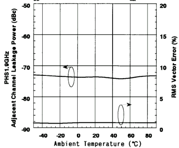
ACP, RMS VECTOR ERROR vs. TEMPERATURE ( V_{DD}=3V, f=1.9GHz, \text{offset}=600kHz, P_{out}=+8dBm )
