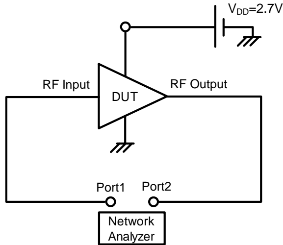
S parameter Measurement Block Diagram
