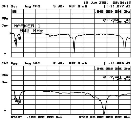
S11, S22
