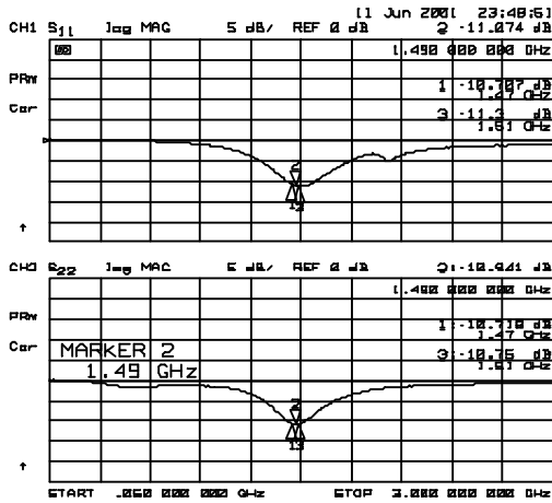
S11, S22
