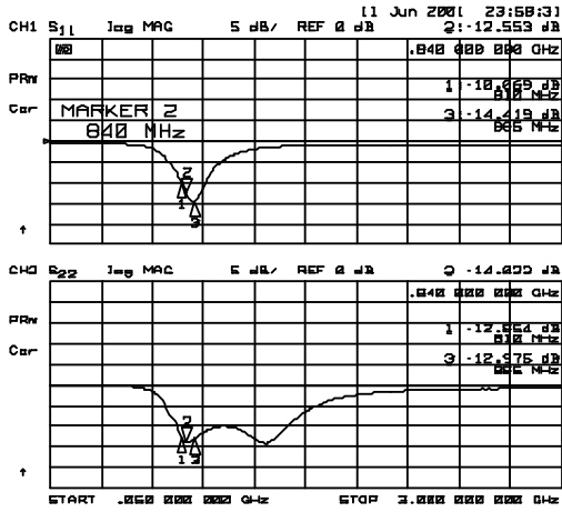
S 11 , S 22
