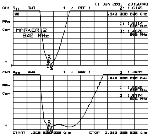
SWR
