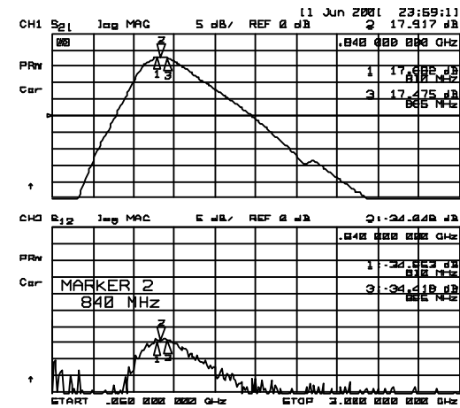
S 21 , S 12
