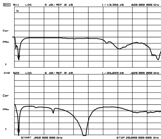
S11, S22 (50MHz~20GHz)
