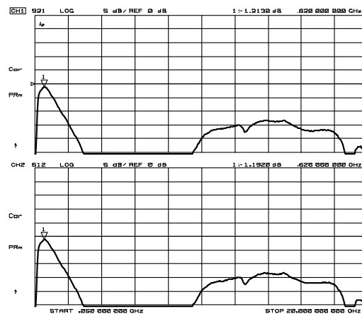
S21, S12 (50MHz~20GHz)
