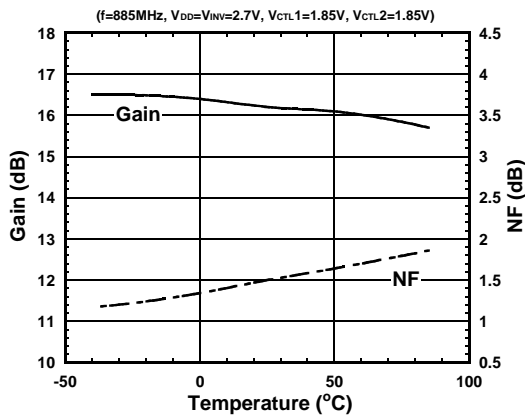
Gain, NF vs. Temperature
