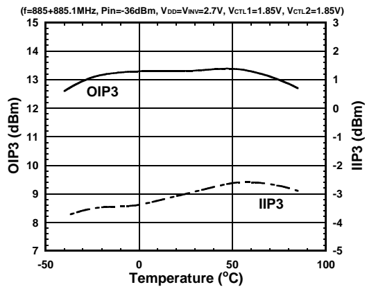
OIP3, IIP3 vs. Temperature
