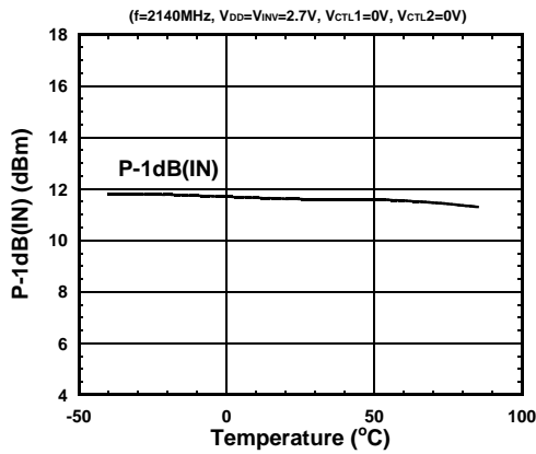
P-1dB(IN) vs. Temperature
